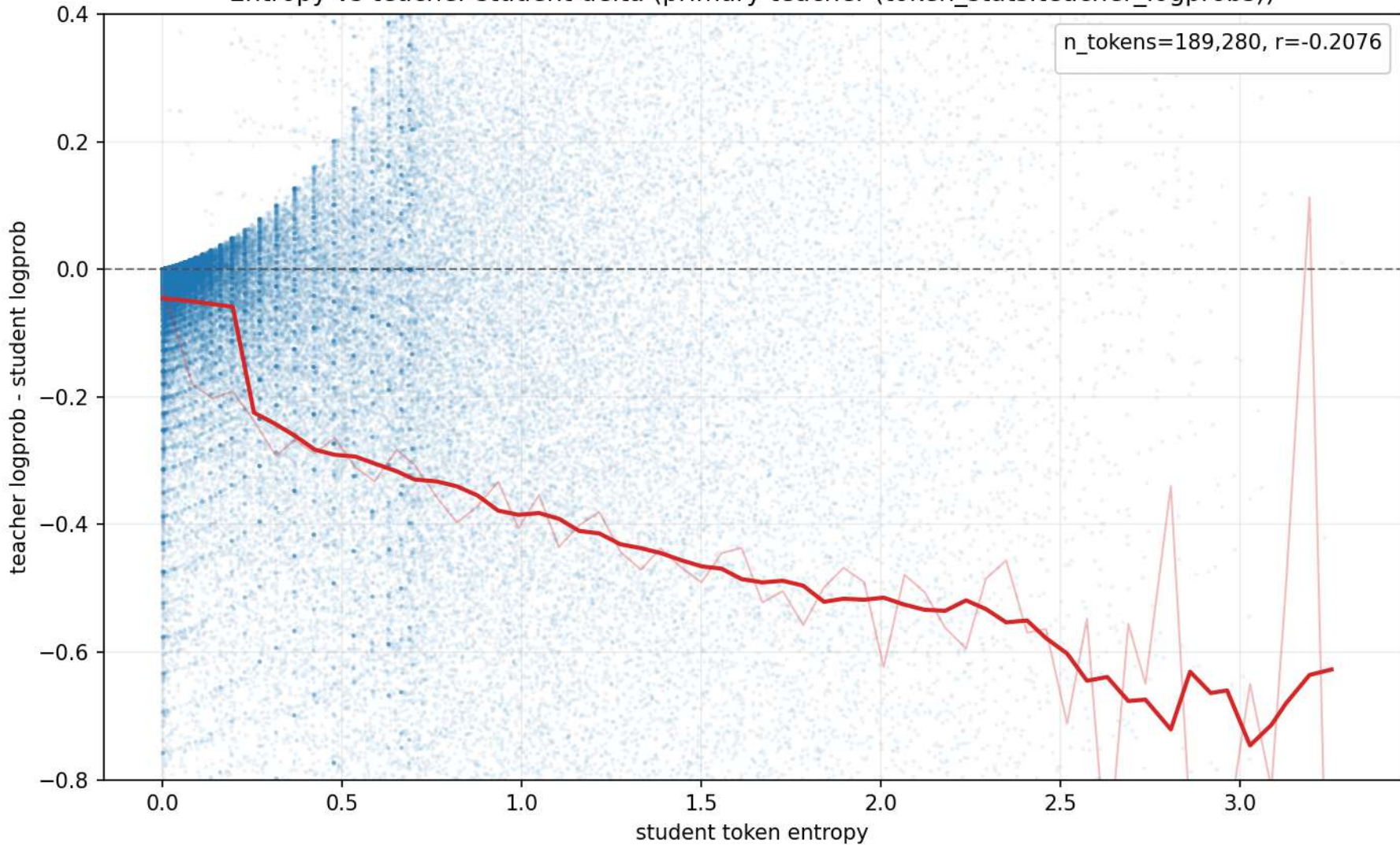
Entropy vs teacher-student delta (primary teacher (token_stats.teacher_logprobs))
